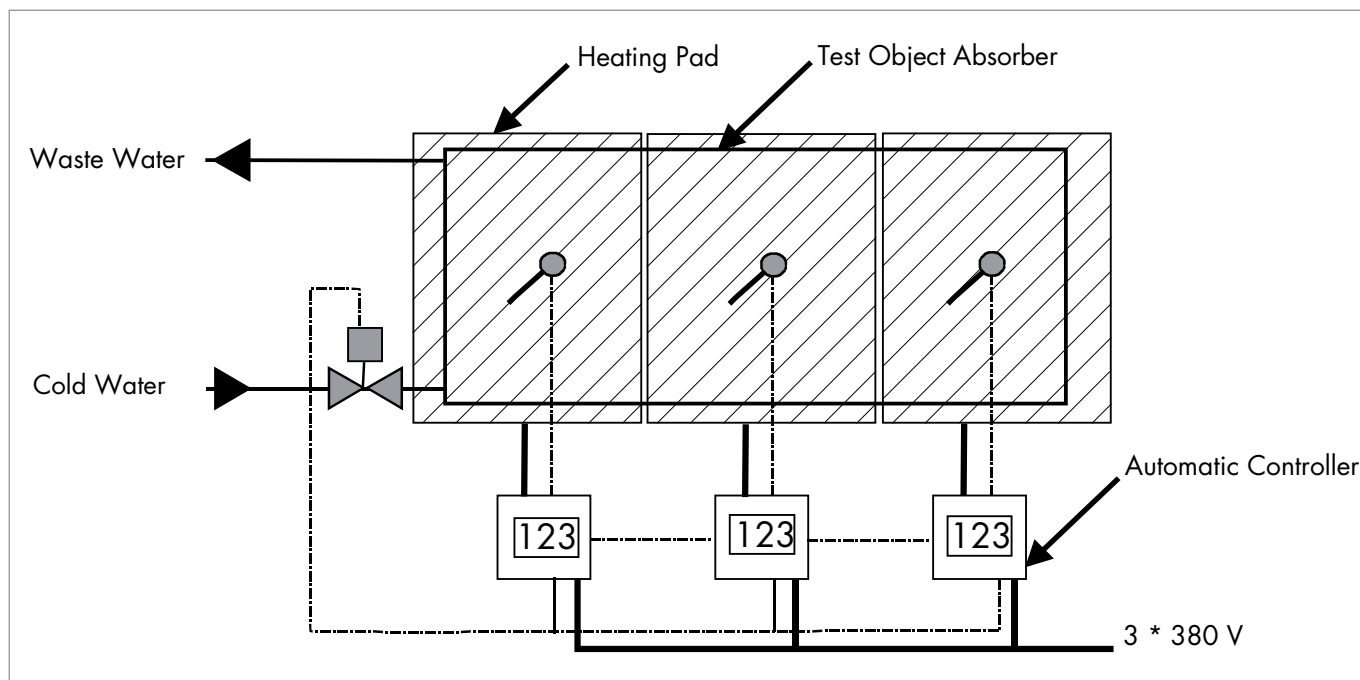
Figure 1: Test setup
