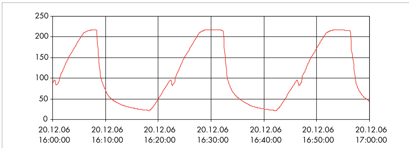
Figure 2: Temperature profile over time of high temperature cycle
