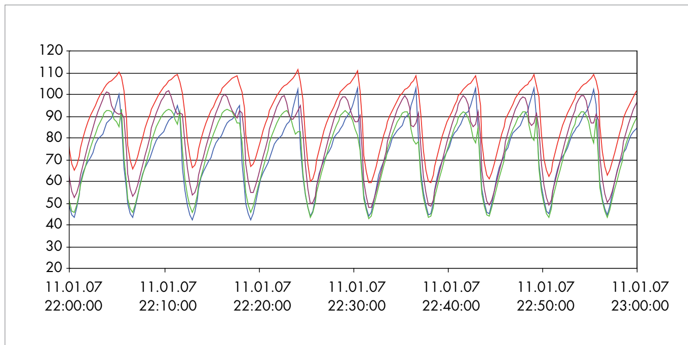
Figure 3: Temperature profile over time of low temperature cycle
