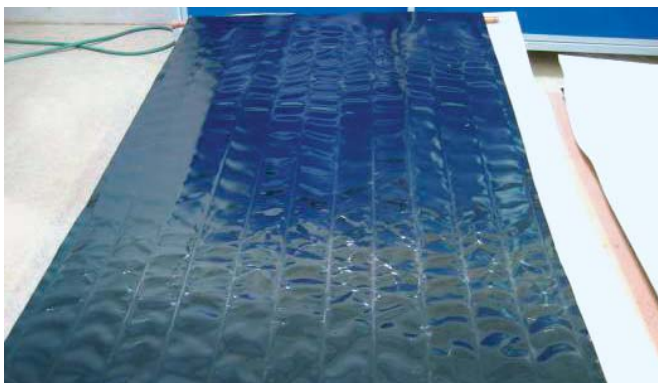
Images 1 and 2: Photo of the absorber after the shock test. Formation of ripples on the absorber plate.
