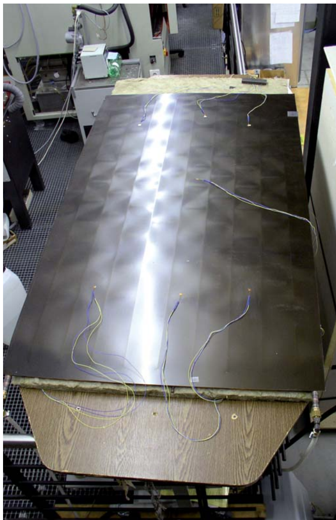
Figure 6: Absorber lying on insulation platform. Various positioned Pt100 sensors visible on absorber surface.
