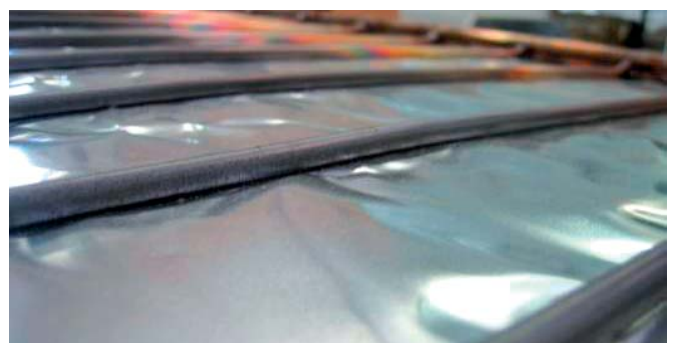
Images 1 and 2: Photo of the absorber after the shock test. Formation of ripples on the absorber plate.
